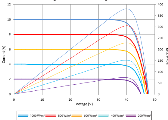
Current-Voltage & Power-Voltage Curve (380S)
